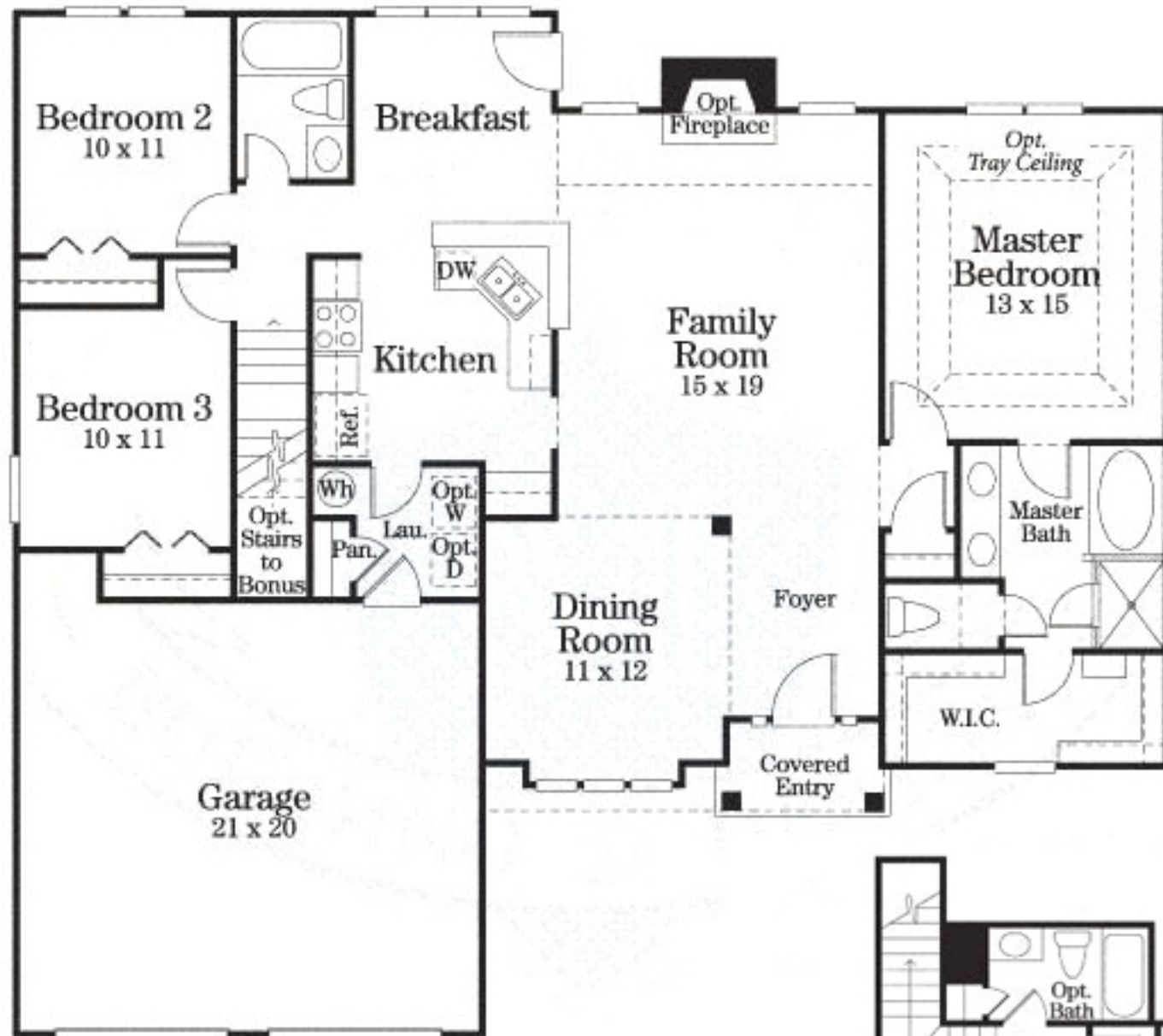
FIRST FLOOR
